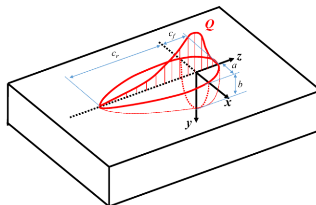
Figure 2. Longitudinal residual stress distribution near the weld toe for different welding heat input levels.
