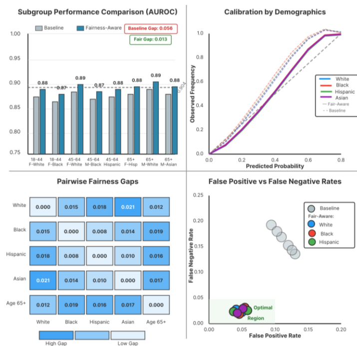
Figure 3. Demographic subgroup performance analysis and fairness comparisons.
