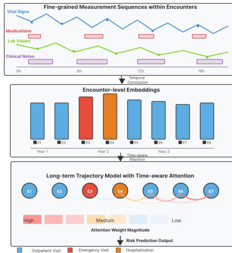
Figure 1. Hierarchical temporal attention architecture for multimodal health data integration.
