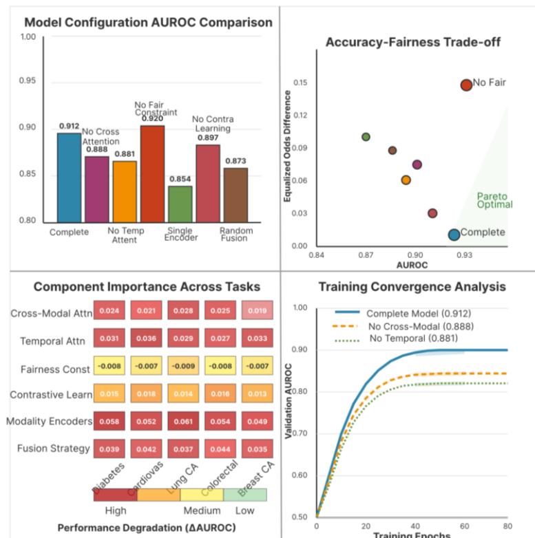
Figure 2. Ablation analysis of architectural components and their impact on performance.
